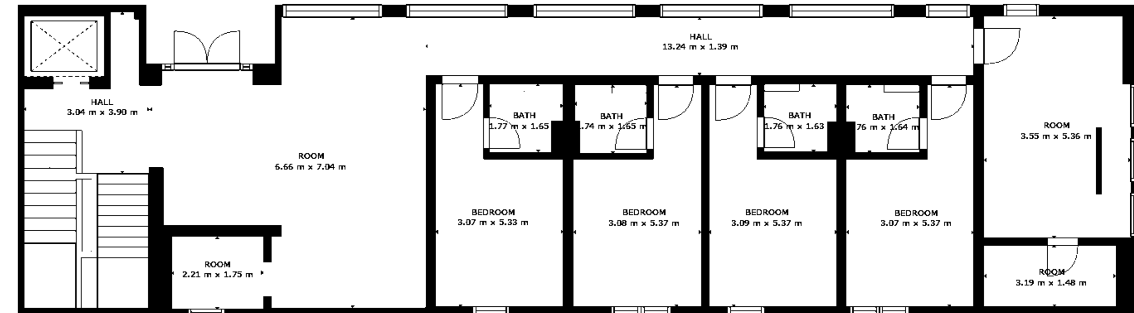
FLOOR 2
