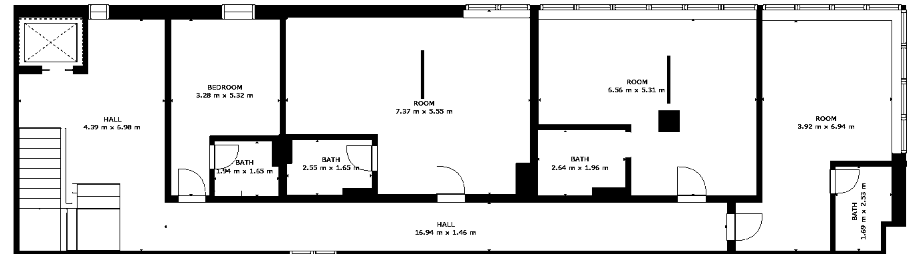
FLOOR 4
